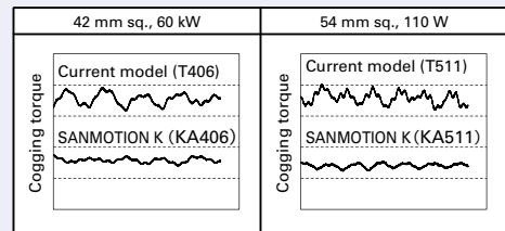
■ Comparison of cogging torque waveforms Ideal for inspection equipment that moves at low speeds.
