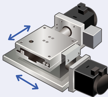
Alignment stage positioning
