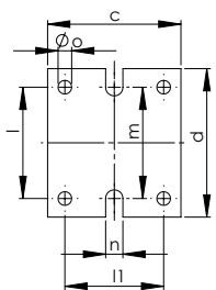
View A Base plate for all types
