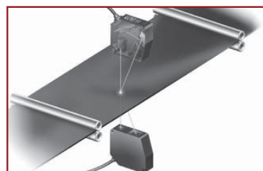
Measuring the thickness of a rubber sheet
