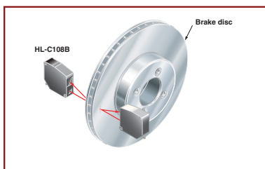
Measuring brake disk thickness
