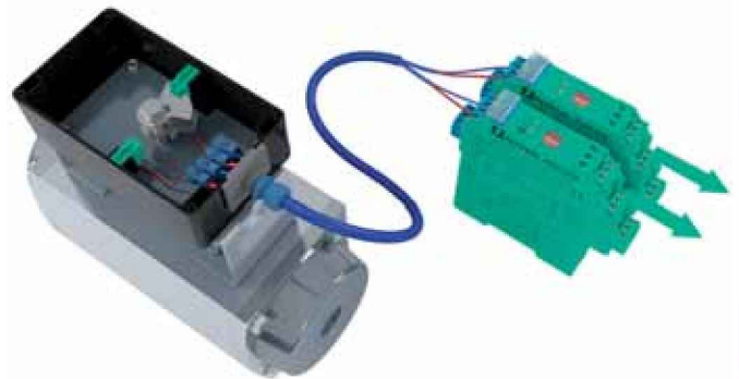
Classic wiring with 2 isolated NAMUR circuits and 2 switch amplifiers
