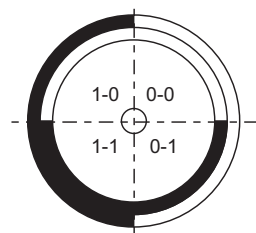
2 bit optic disc with Gray code
