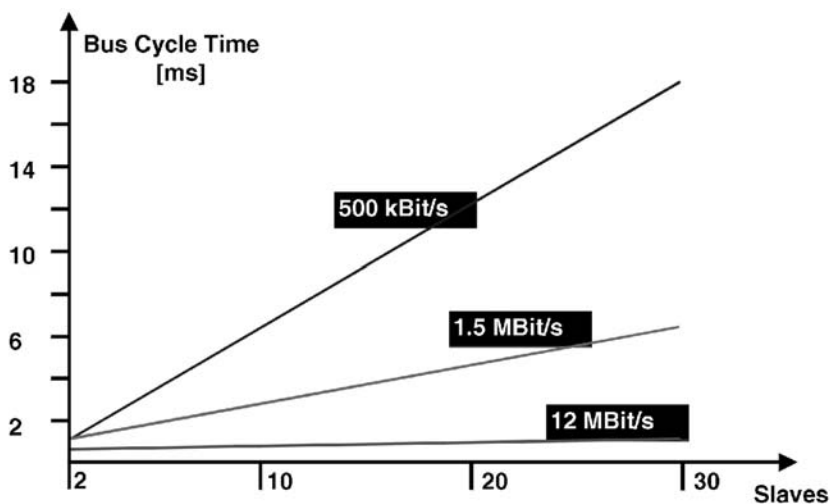
CYCLE TIMES WITH A DP MONO-MASTER NETWORK
